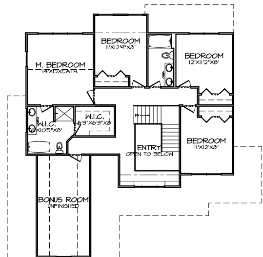
1 SECOND FLOOR PLAN A-5
