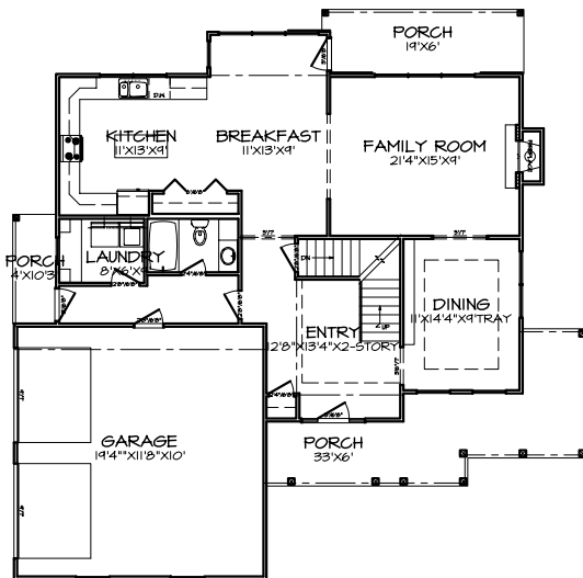
1 FIRST FLOOR PLAN A-4
