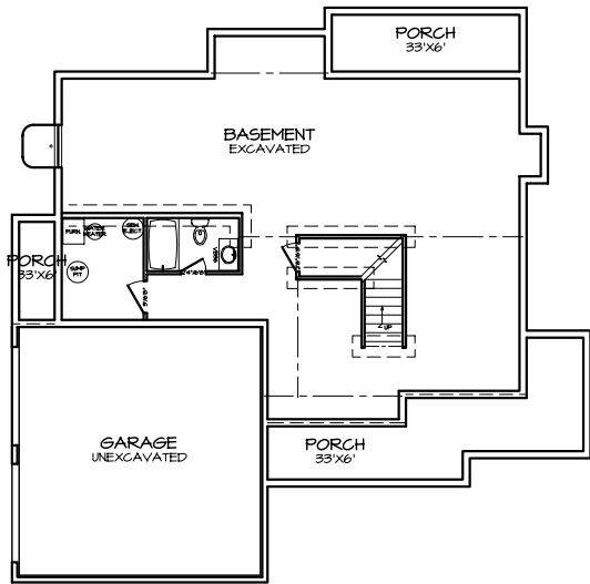
1 FOUNDATION PLAN A-3
